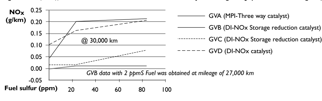
Figure 4: Sulfur effect on Low emission vehicles – Direct Fuel injection engines (Japan Clean Air Program)
