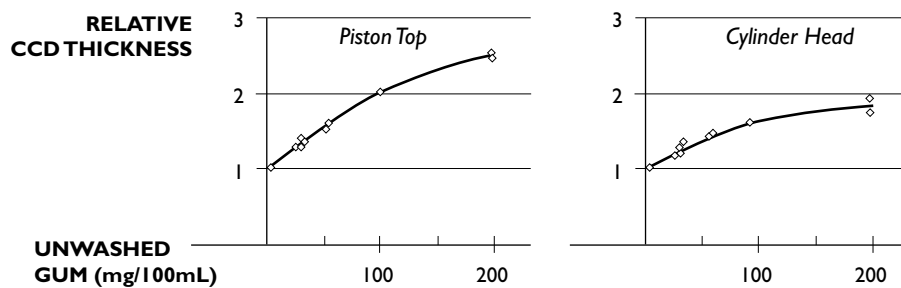
Figure 22: Relationship Between Unwashed Gum and CCD Thickness
